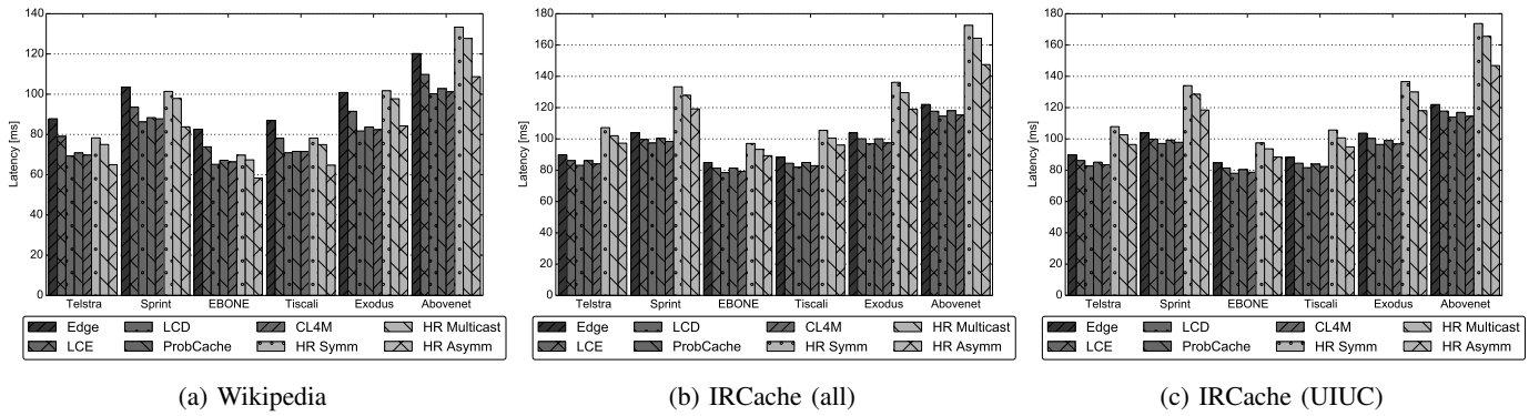
Fig. 6: Latency
